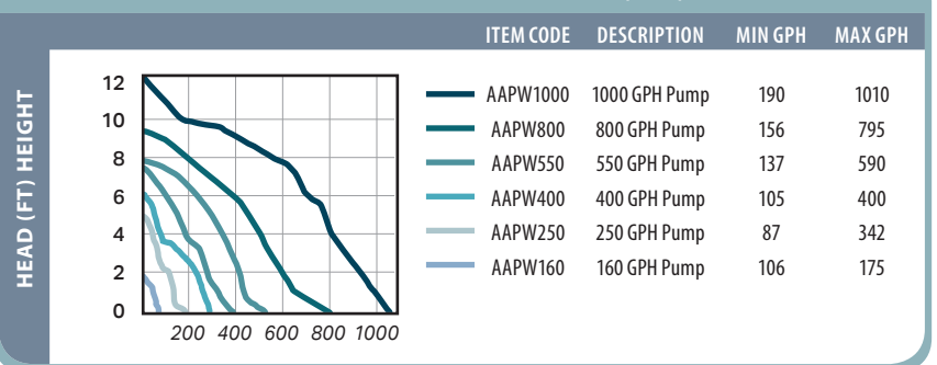
HEAD HEIGHT CHART – FLOW RATE (GPH)
