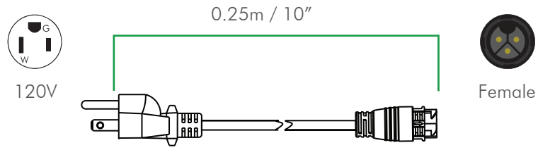
120V AC POWER NEMA 5-15 PLUG IL-T120
